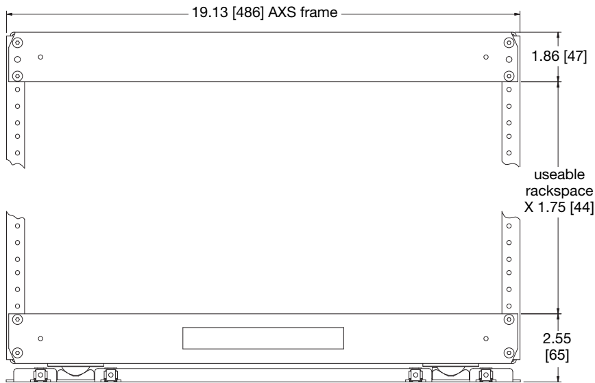
FRONT VIEW (AXS inner frame)
